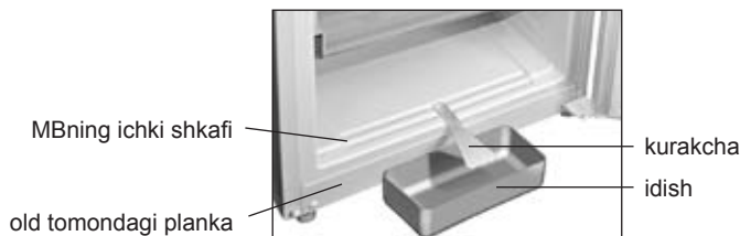
6 Rasm — MBdan erigan suvni yig’ib olish
